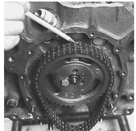
Figure 2 - Check alignment of chain to ensure that both sprockets are correctly installed
